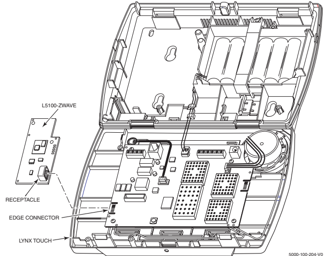
Figure 2. Installing the L5100-ZWAVE Communications Module
